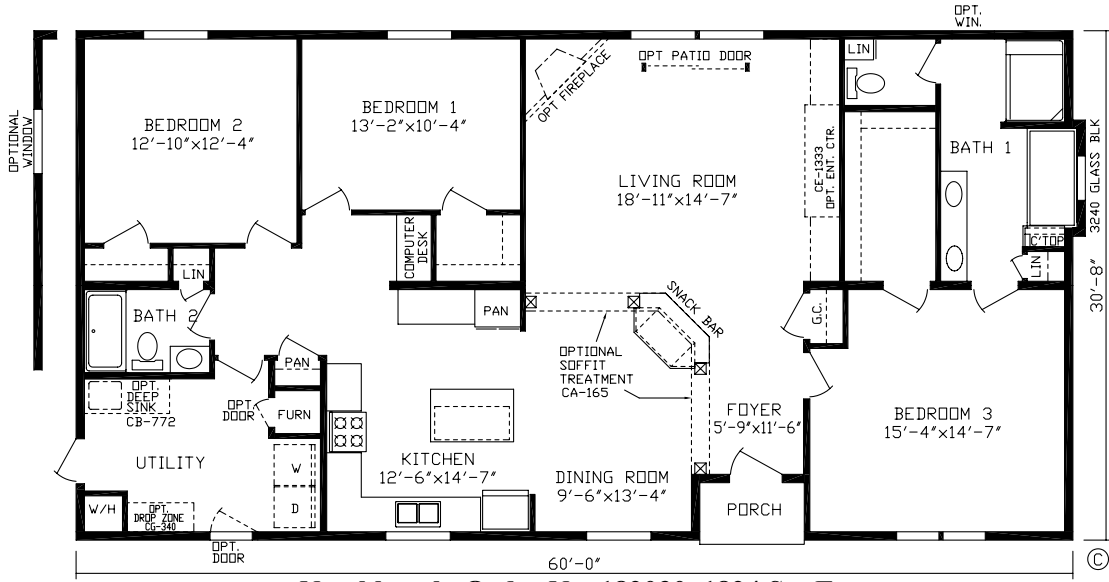
Northbrook Order No. 182030 1824 Sq. Ft. 5/12 Roof, Trane Furnace, & Architectural Shingles Standard in this Home
