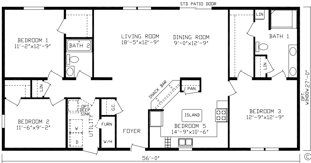
Melbourne Order No. 182014 1512 Sq. Ft.
