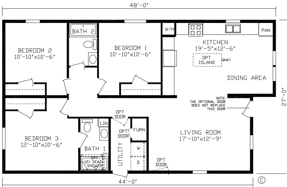
Edgewood Order No. 182007 1242 Sq. Ft.
