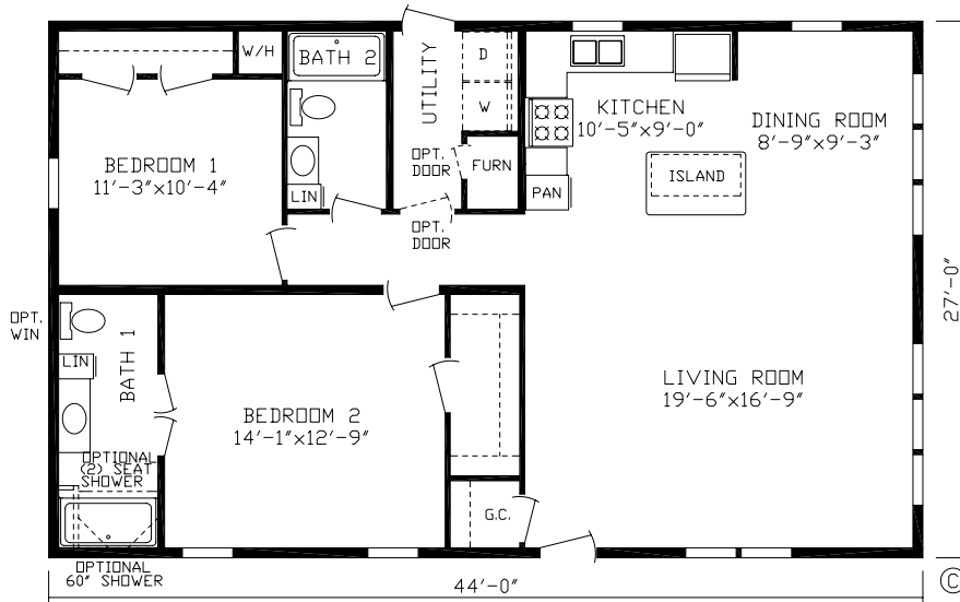
Aurora Order No. 182004 1188 Sq. Ft.
