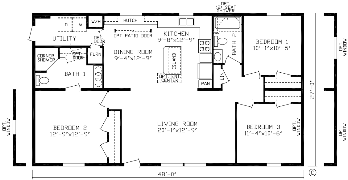
Monroe Order No. 182008 1296 Sq. Ft.
