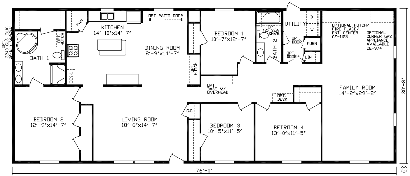
Knollwood Order No. 182031 2330 Sq. Ft. 5/12 Roof, Trane Furnace, & Architectural Shingles Standard in this Home
