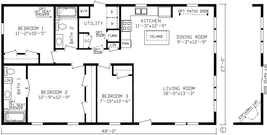
Gifford Order No. 182006 1296 Sq. Ft.
