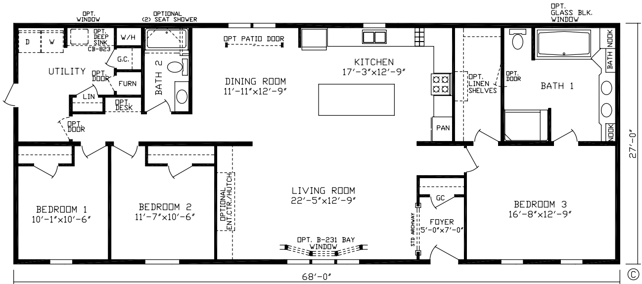
Sea Island Order No. 182023 1836 Sq. Ft.
