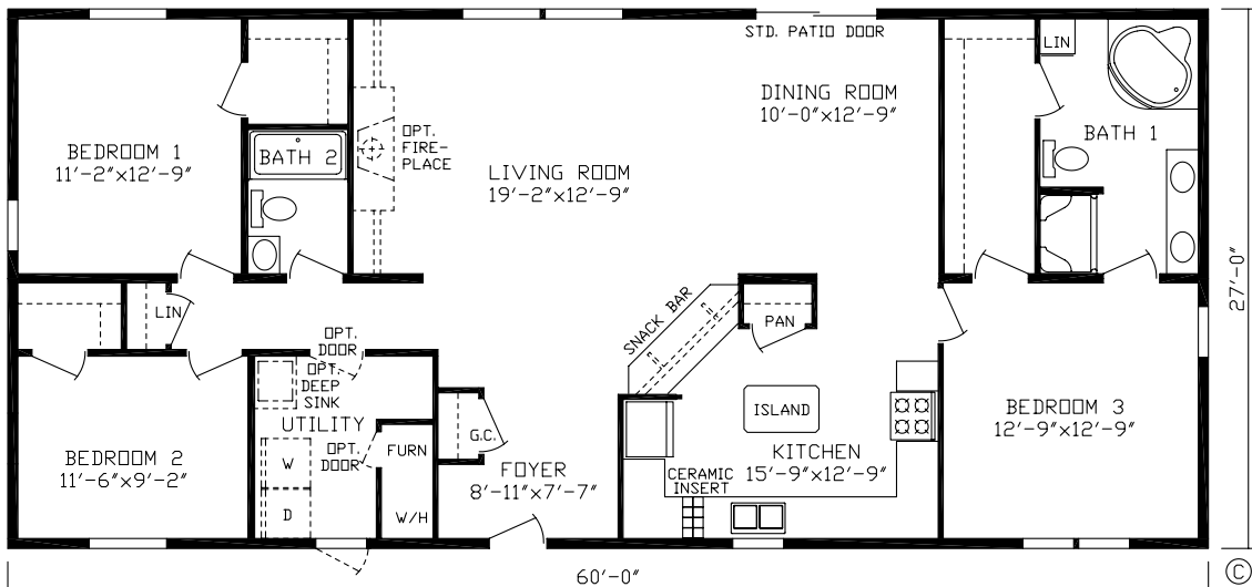
Prescott Order No. 182017 1620 Sq. Ft.
