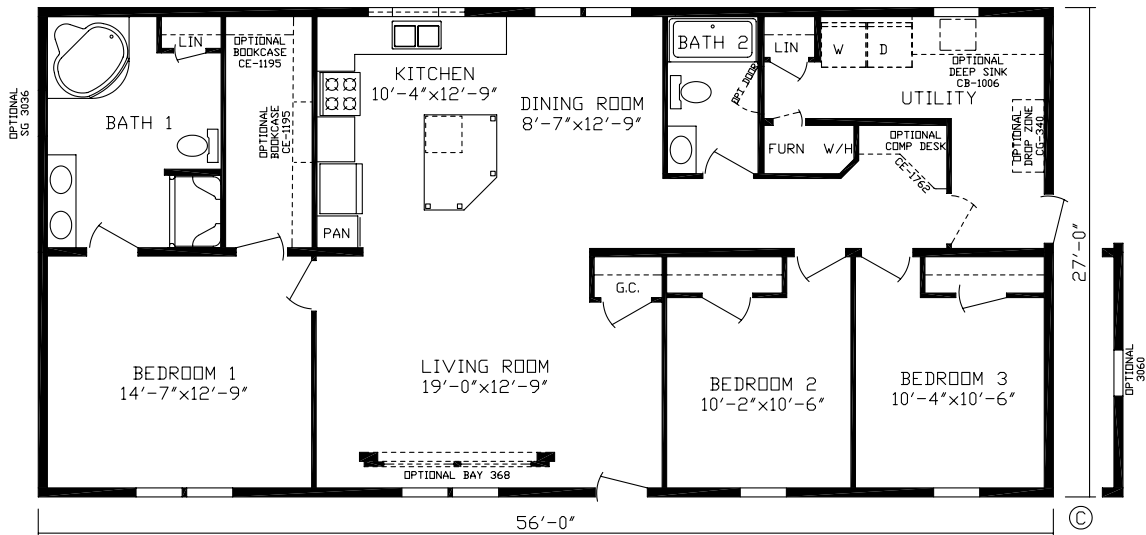
Hinsdale Order No. 182016 1512 Sq. Ft.
