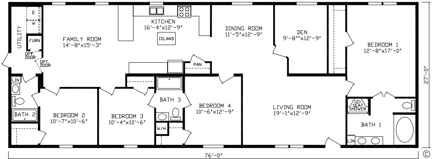
Warren Order No. 182026 2052 Sq. Ft.
