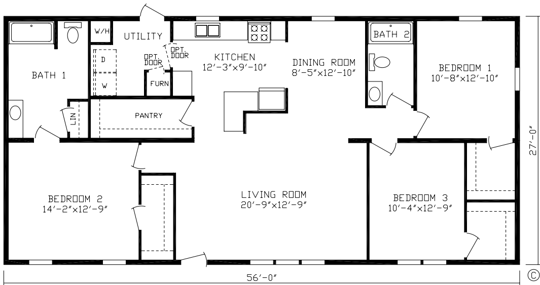
Walden Order No. 182035 1512 Sq. Ft.
