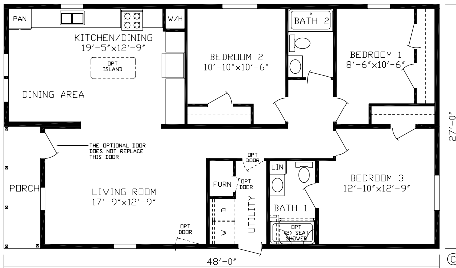
Hudson Order No. 182005 1242 Sq. Ft.
